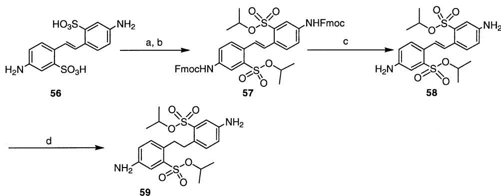
Scheme 2. Preparation of stilbene and dihydrostilbene (bis)sulfonic acid, diisopropyl esters: (a) Fmoc-Cl, Na 2 CO 3 , dioxane, water; (b) HC(OiPr) 3 , dioxane, 110 °C, 82% (two steps); (c) piperidine, DMF, 0 °C, 80%; (d) H 2 , Pd/C, THF, 85%.
