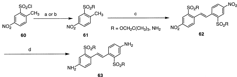
Scheme 3. Preparation of stilbene (bis)sulfonic acid, dinepentyl esters and (bis)sulfonamides: (a) R = OCH 2 C(CH 3 ) 3 : HOCH 2 C(CH 3 ) 3 , pyridine, dioxane, reflux, 55%; (b) R = NH 2 : aq NH 4 OH, ether, 0 °C, 38%; (c) KOtBu, DMF, air, 53% for R = OCH 2 C(CH 3 ) 3 , 21% for R = NH 2 ; (d) SnCl 2 , ethyl acetate, 73% for R = OCH 2 C(CH 3 ) 3 , 31% for R = NH 2 .
